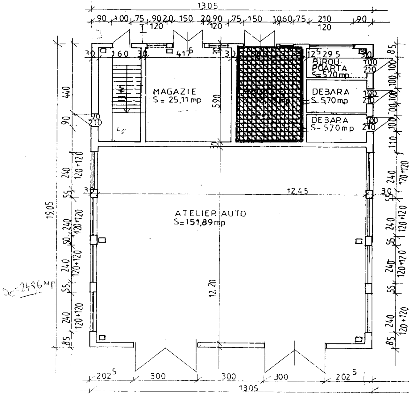
PLAN 'PARTER RELEVU SC 1:100
